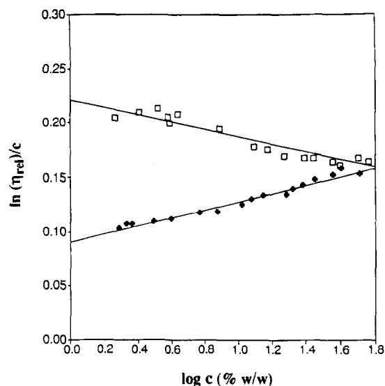
Fig. 11. Concentration dependence of (\ln \eta_{rel})/c for mesquite gum (+) and gum arabic (□) at 20°C in 0.1 M NaCl.
