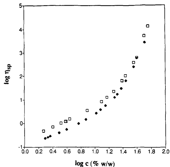
Fig. 10. Concentration dependence of specific viscosity (20°C; 0.1 M NaCl) for mesquite gum (+) and gum arabic (□).
