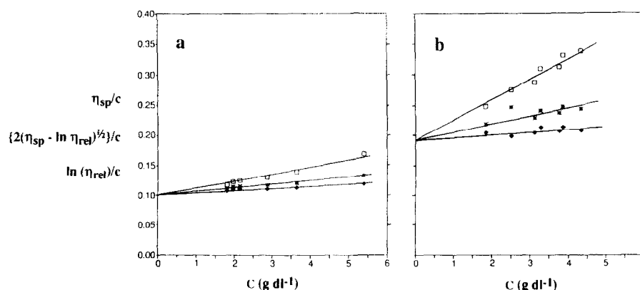
Fig. 4. Determination of intrinsic viscosity ( 20^\circ\text{C} ; 0.1 M NaCl) for: (a) mesquite gum; and (b) gum arabic by combined Huggins (□), Kraemer (+) and single-point (*) extrapolation of, respectively, \eta_{\text{sp}}/c , (\ln \eta_{\text{rel}})/c and \{2(\eta_{\text{sp}} - \ln \eta_{\text{rel}})\}^{1/2}/c to zero concentration.
