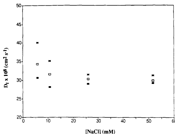
Fig. 1. Variation of translational diffusion coefficient ( D_t ) with salt (NaCl) concentration for mesquite gum at polymer concentrations (% w/w) of 0.10 (■), 0.25 (□) and 0.50 (*). Measurements were made at \sim 26.8^\circ\text{C} (300 K).
