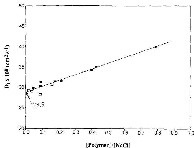
Fig. 2. Diffusion coefficients from Fig. 1, plotted as a function of the molar ratio of the concentration of negatively charged groups on mesquite gum to the concentration of surrounding cations. Symbols as in Fig. 1.
