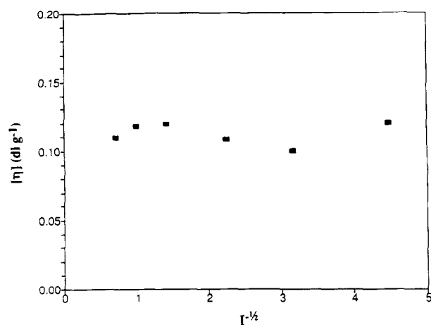
Fig. 5. Variation of intrinsic viscosity (20°C) with ionic strength ( I ) for mesquite gum dialysed to equilibrium against NaCl solutions with concentrations ranging from 0.05 to 2.0 M.
