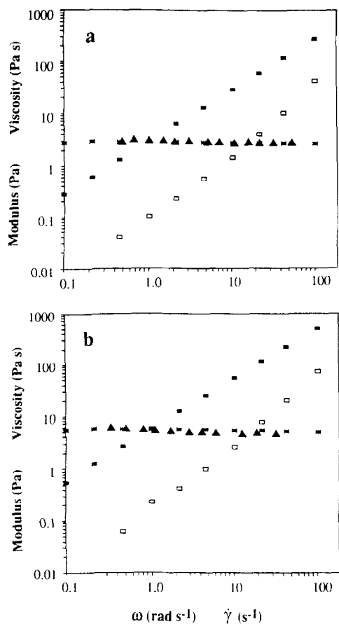
Fig. 7. Mechanical spectra (20°C; 0.1 M NaCl) for 50% w/w solutions of: (a) mesquite gum; and (b) gum arabic, showing the variation of G' ( \square ), G'' ( \blacksquare ) and \eta^* (*) with frequency ( \omega ). The dependence of steady shear viscosity ( \eta ) on shear rate ( \dot{\gamma} ) is also shown ( \blacktriangle ).
